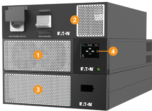
Front of 5 and 7.5 kW UPS (9U)
