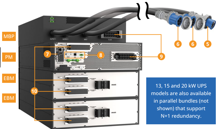
Back of 13 and 15 kW UPS (20 kW UPS is similar, but with hardwired input. Hardwired input and output are also available for 13, 15 and 20 kW UPS systems.)
