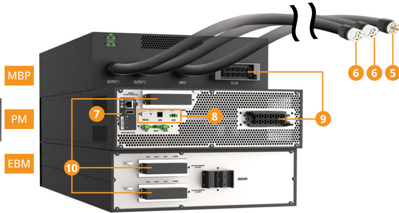
Back of 5 kW UPS (7.5 kW UPS is similar, but with 30A input/output instead of 20A.)
