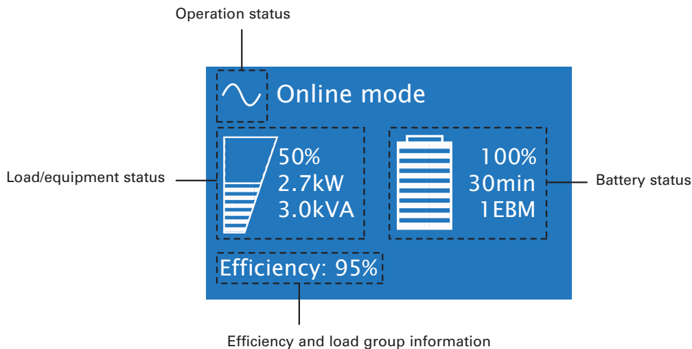
Figure 4. LCD Description
