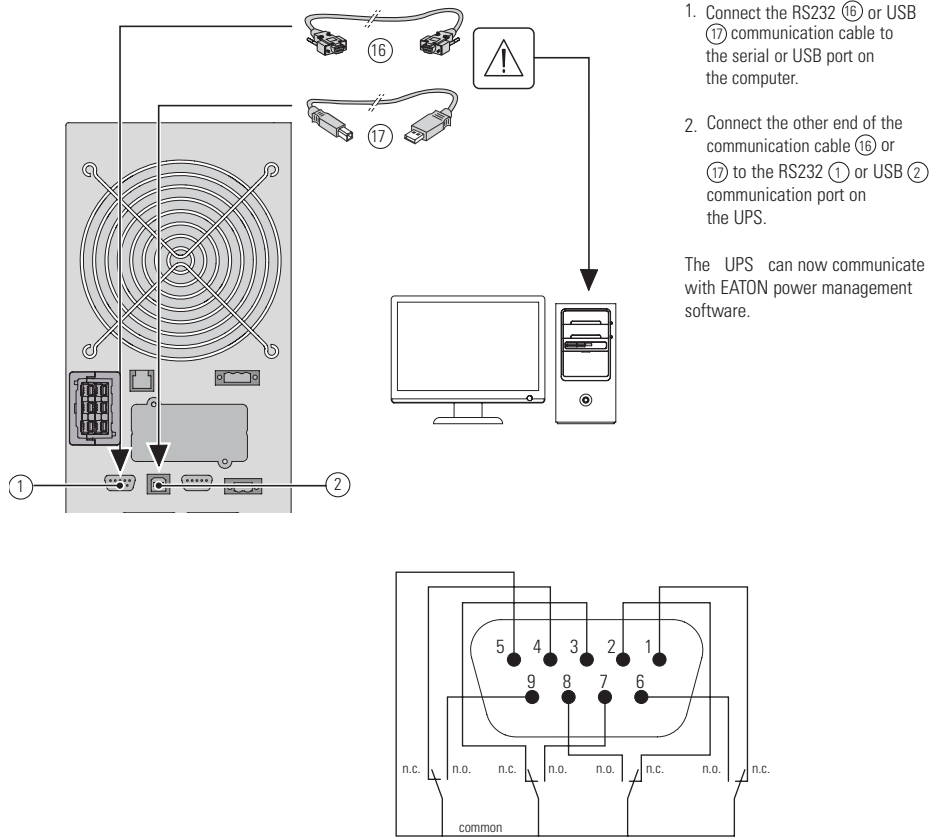
Figure 12. Communication Port Information
