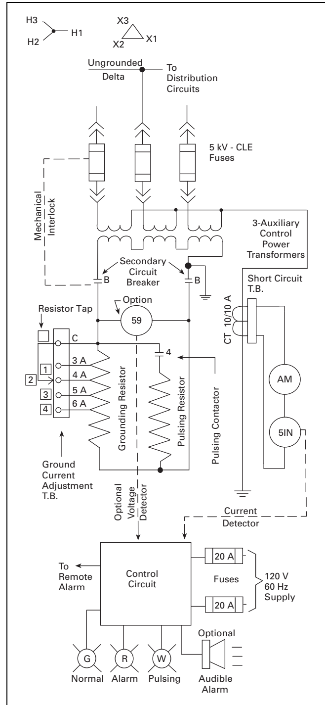
Figure 36.1-3. Ungrounded Delta System (With Standard Current and Optional Voltage Relay Fault Detectors)
