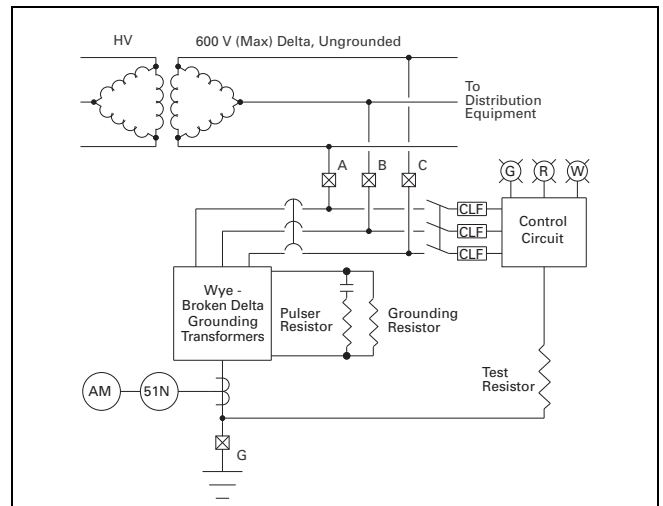
Figure 36.2-7. Three-Wire Source—Fault Detection via Current Relay
