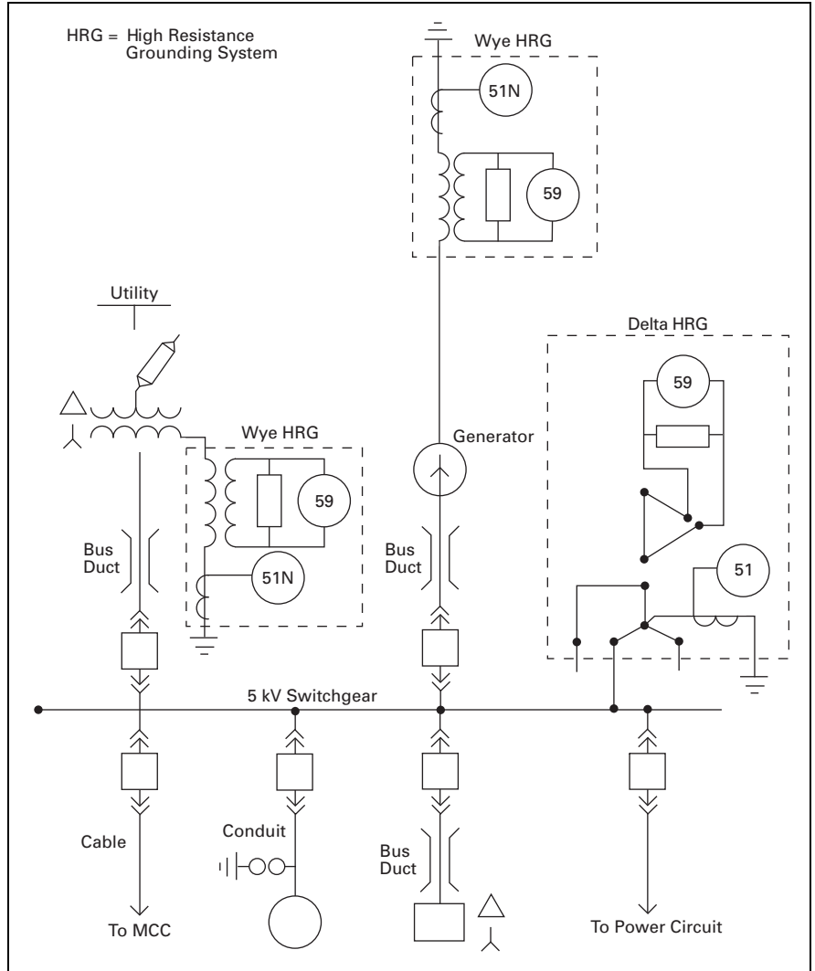
Figure 36.1-1. HRG—High Resistance Grounding System
