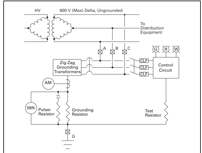
Figure 36.2-6. Three-Wire Source—Fault Detection via Voltmeter Relay
