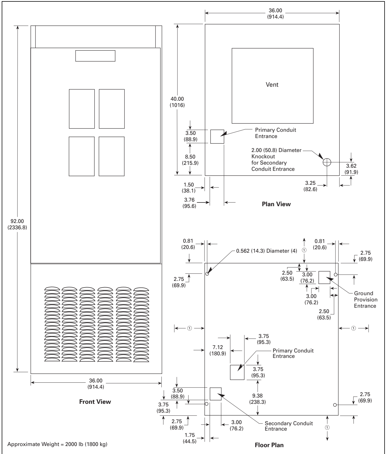
Figure 36.1-4. NEMA 1 Free-Standing
