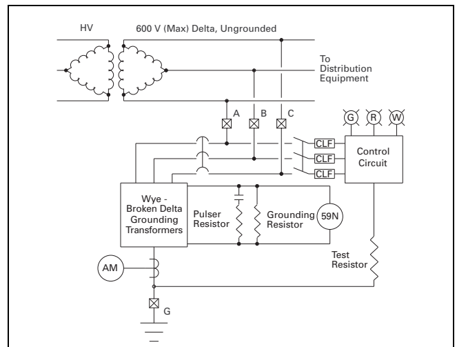
Figure 36.2-8. Three-Wire Source—Fault Detection via Voltmeter Relay
