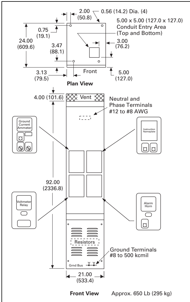
Figure 36.2-9. NEMA 1 Free Standing
