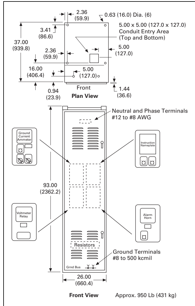
Figure 36.2-10. NEMA 3R Outdoor
