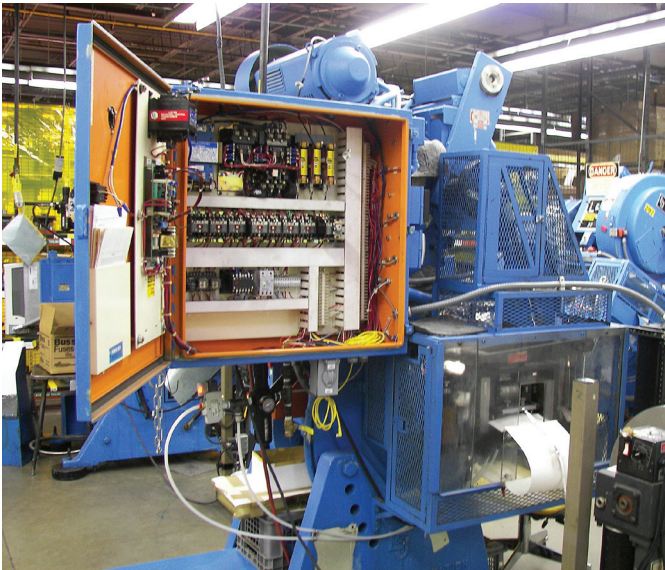
This machine's industrial control panel has 50 kA SCCR marked on the nameplate inside the enclosure. The available short-circuit current is field marked on the exterior.
