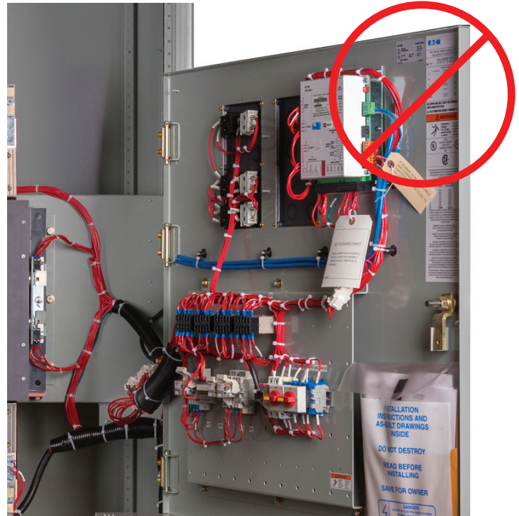
An SCCR field marking for the specific installation of emergency system transfer equipment must be made on the enclosure exterior — not the interior. The manufacturer's nameplate SCCR marking is on the inside
