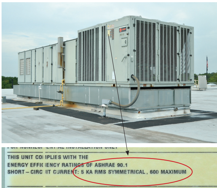
HVAC units cannot be installed where the available short-circuit current is greater than the equipment SCCR. The unit above would be a Code violation if installed at "HVAC Rooftop — North" as summarized in the report shown in Figure 3.
