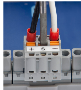
Figure 5.2: Spring Clamp
